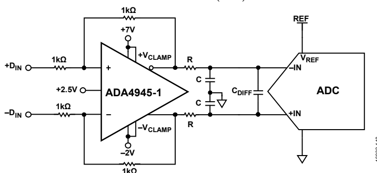
Figure 116. ADA4945-1 Driving Precision ADC
