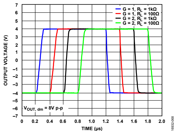
Figure 88. Large Signal Transient Response for Various Gains and Loads
