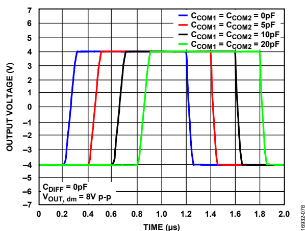
Figure 89. Large Signal Transient Response for Various Capacitive Loads, V_S = 10\text{ V}
