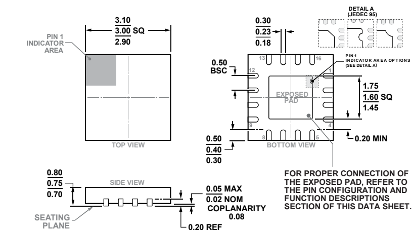
Figure 117. 16-Lead Lead Frame Chip Scale Package [LFCSP] 3 mm × 3 mm Body and 0.75 mm Package Height (CP-16-22)
