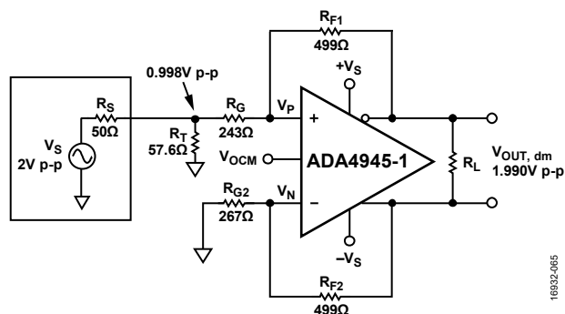
Figure 109. Terminated Single-Ended-to-Differential System with G = 1
