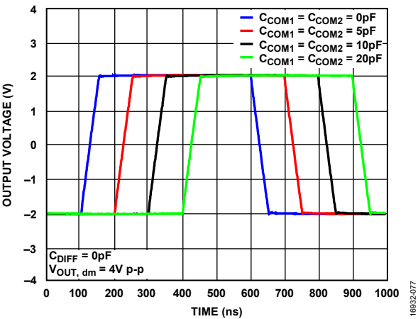
Figure 46. Large Signal Transient Response for Various Capacitive Loads, V_S = 3\text{V}
